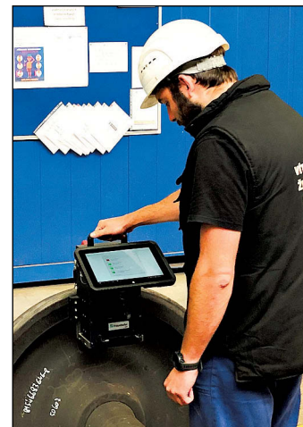
A mobile measurement of wheelset internal stress
